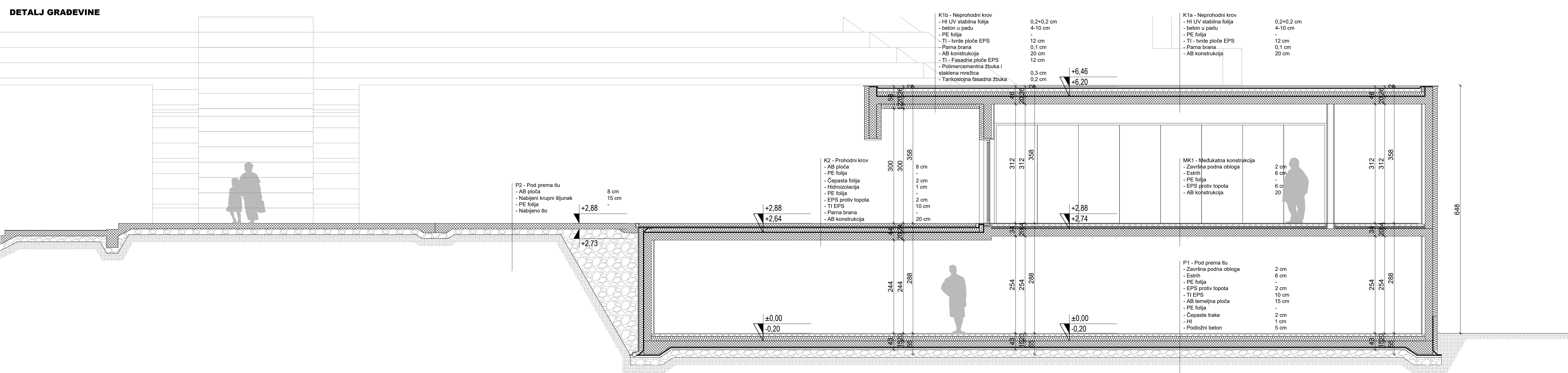
DETALJ GRADEVINE
