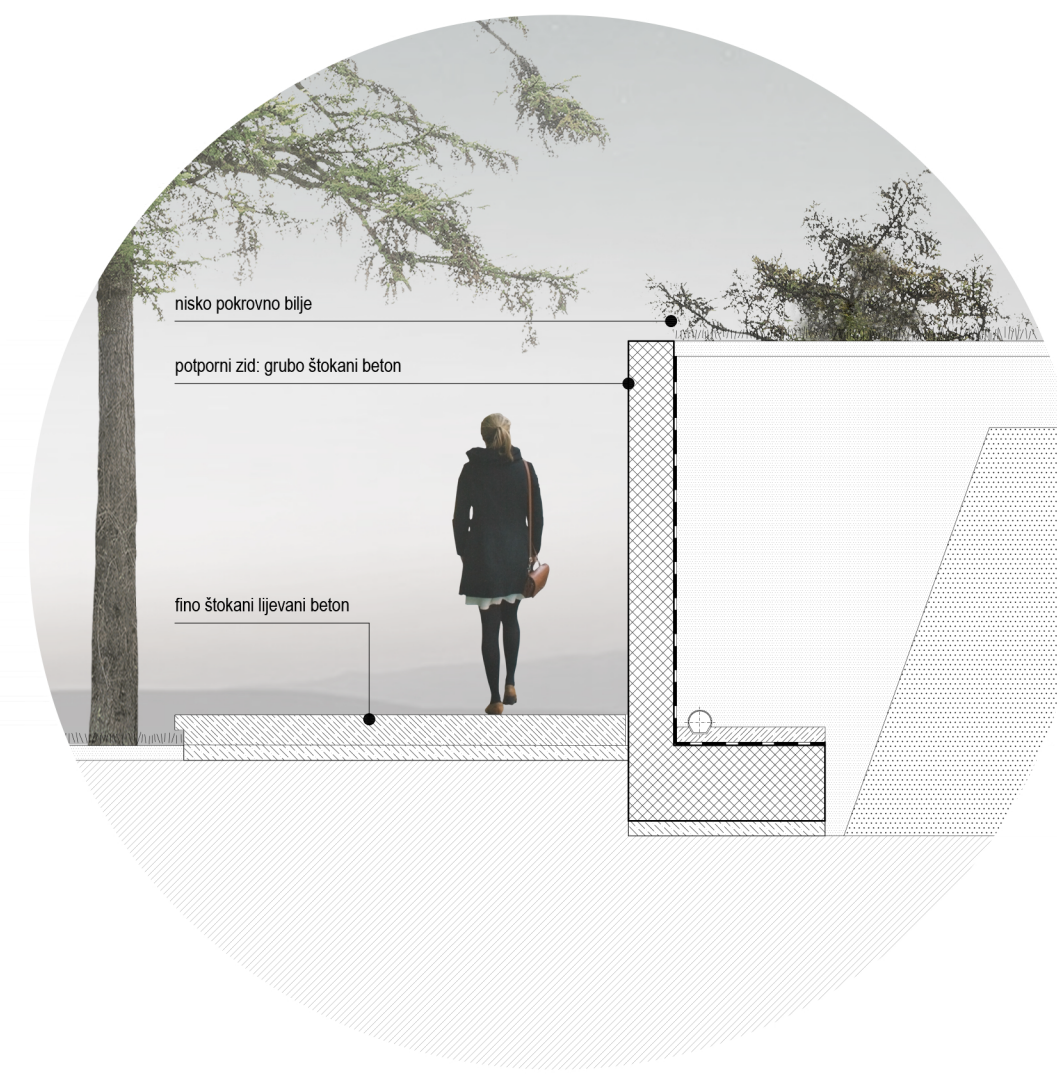
Detaji reliefnog oboda M 1:50
